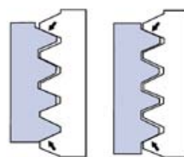
Pitch and Angle Error Compensation Problems
